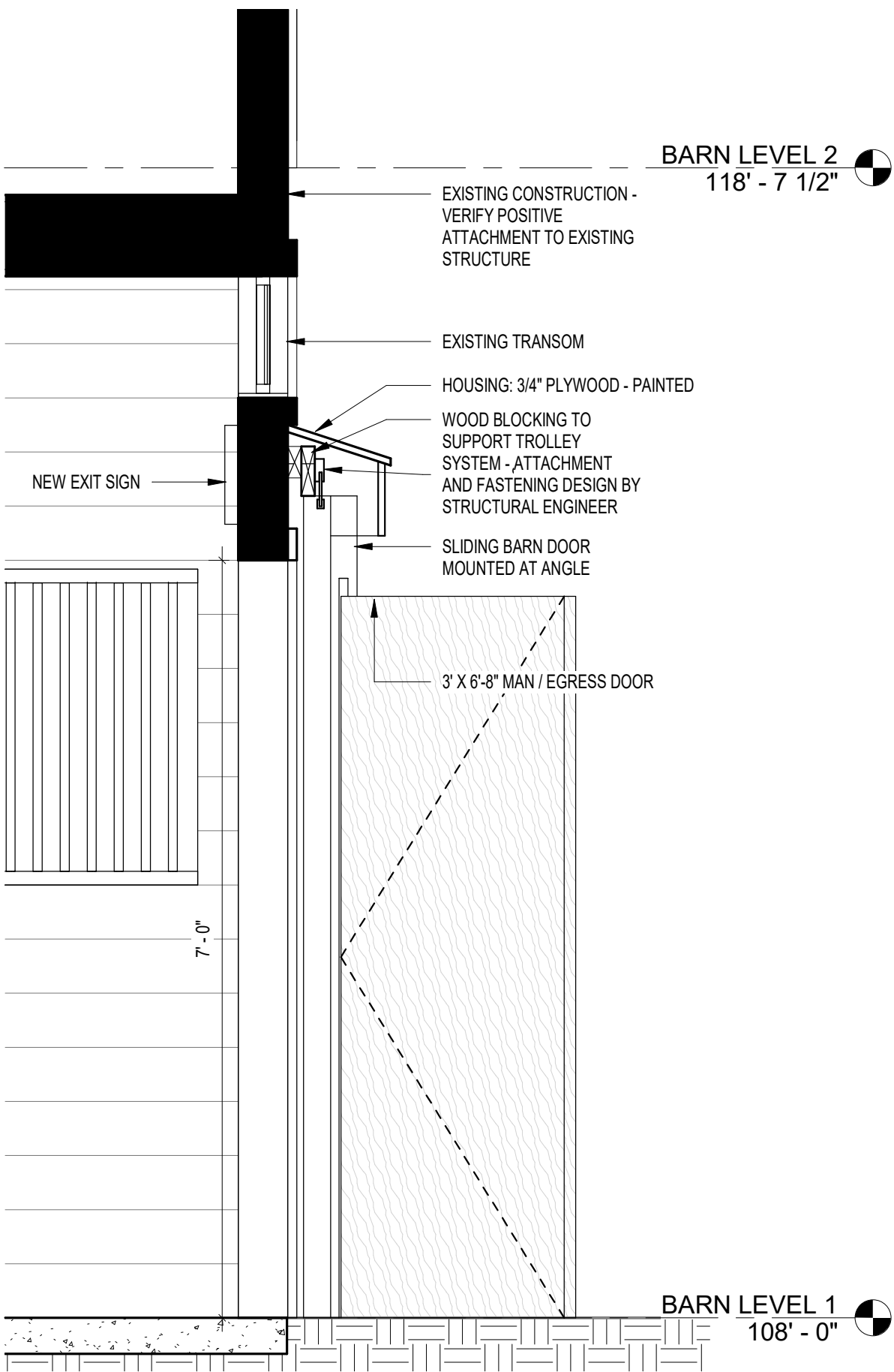
SECTION THROUGH NEW SLIDING DOOR 3/4" = 1'-0"
